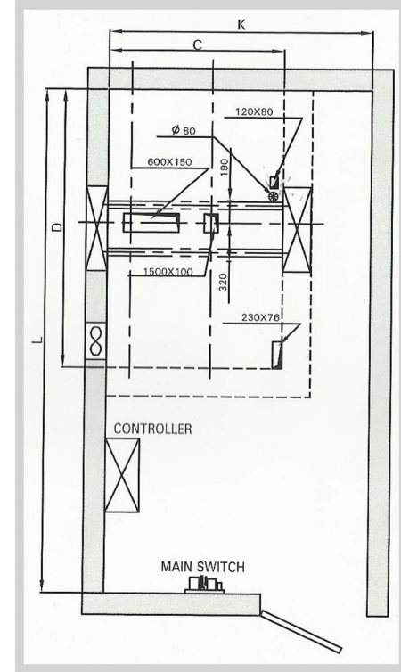
MACHINE ROOM PLAN
